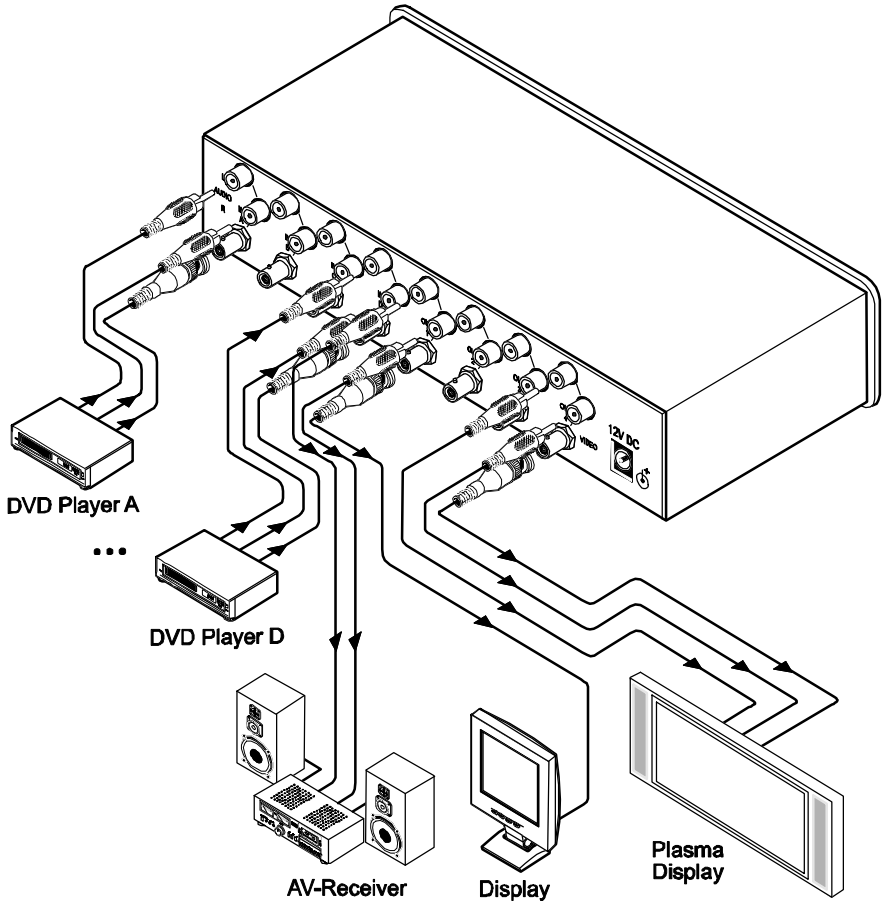
Figure 2: VS-6EIII 4x4 Video Audio Matrix Switcher Connections
