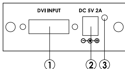
Front Panel
